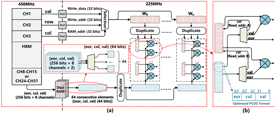
Fig. 28. Fully pipelined general purpose computing engine in Graph-OPU [4]: (a) the architecture of computational engine; (b) the architecture of PE units is connected to a selective adder tree.
