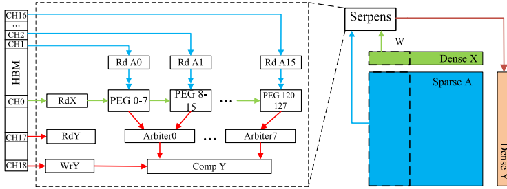
Fig. 15. Overall architecture of Serpens within [57].
