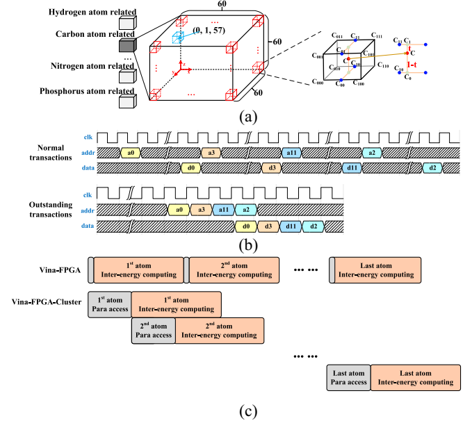
Fig. 12. (a) Diagram of trilinear interpolations for inter-molecular energy calculation. (b) Different transactions are used for continuous access to non-continuous addresses. The double wavy lines represent the time taken to establish AXI protocol handshakes. (c) The pipeline access mode of Vina-FPGA-cluster introduces a minimal increase in parameter accessing latency.
