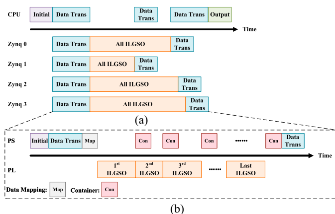
Fig. 10. (a) The scheduling between the CPU and Zynq FPGAs. (b) The scheduling between the PS and PL.
