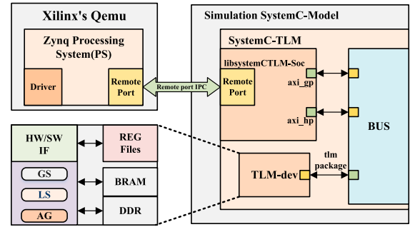
Fig. 5. The SystemC-based SW/HW co-design model.
