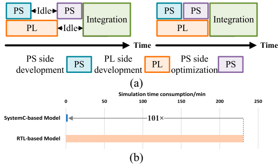
Fig. 6. (a) Comparison of development workflows: traditional RTL model-based co-design (left) requires PS side optimization to wait for PL side completion. SystemC model-based co-design (right) enables simultaneous development without waiting for PL side. (b) Comparison of simulation time consumption under different models.
