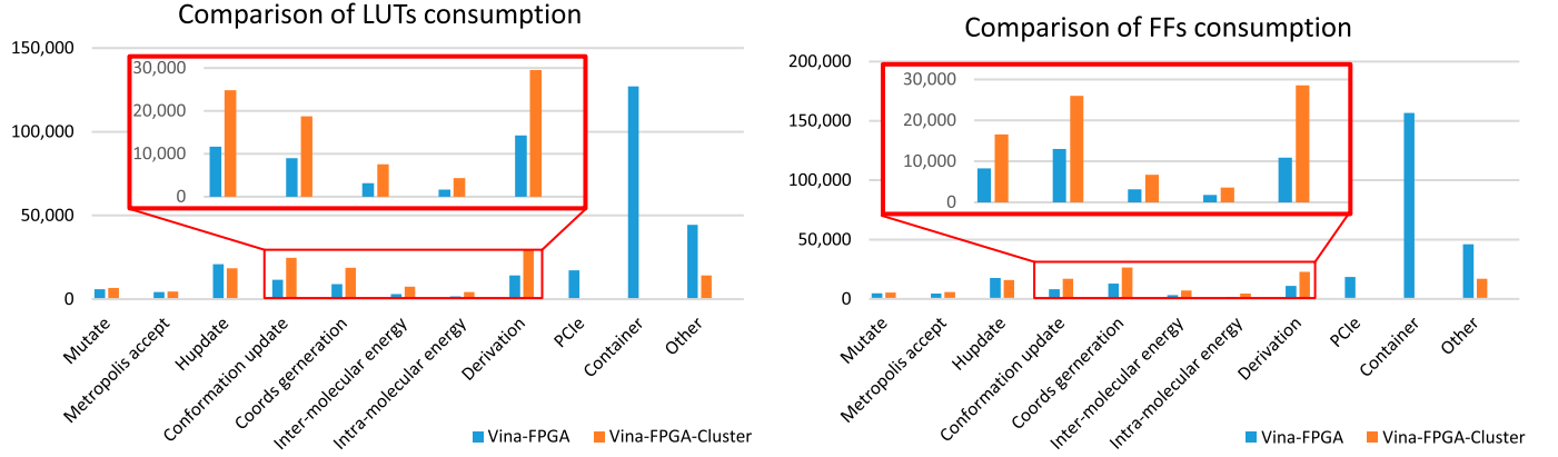
Fig. 17. The basis FPGA resource consumption comparison of Vina-FPGA and Vina-FPGA-cluster (on a single board).
