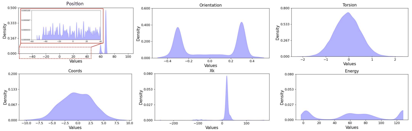
Fig. 3. Probability density functions of Vina computational data.
